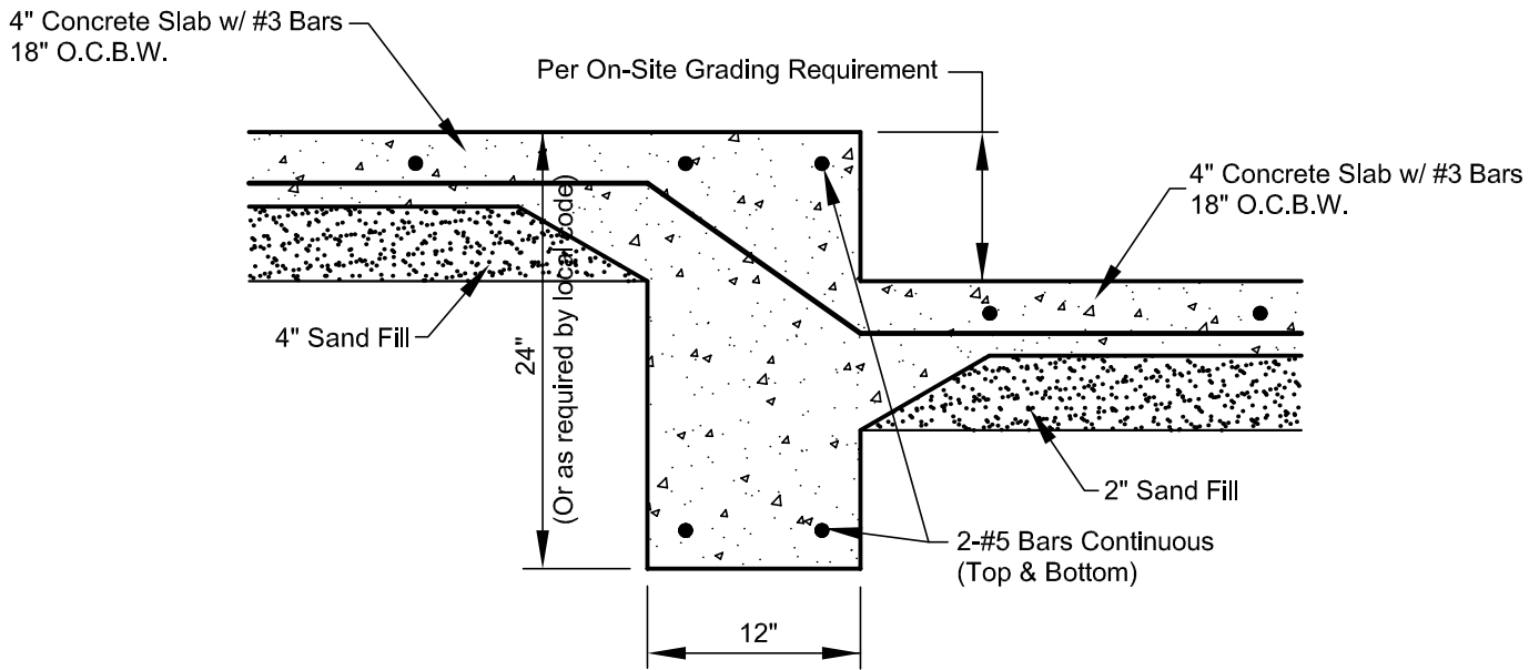
SLAB DROP DETAIL
